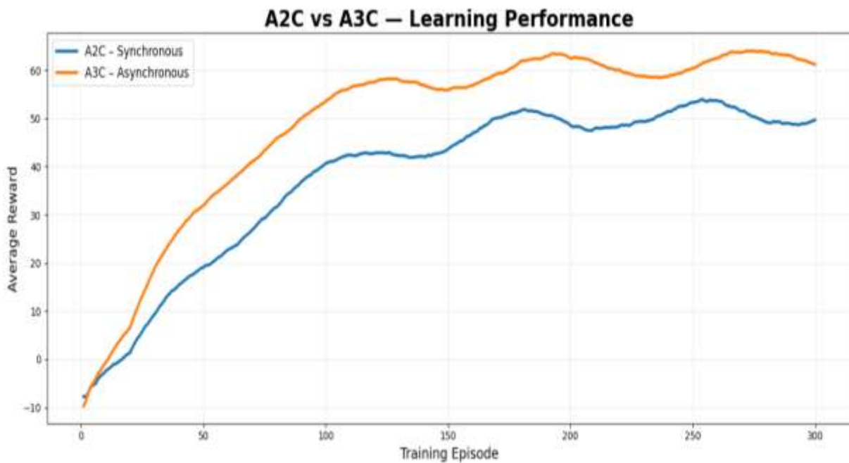
Fig 5: - A2c vs A3C Learning Performance
